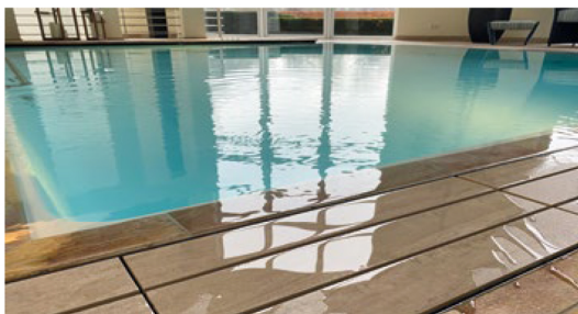
Overflow channel with stone cover adjustable overflow weir of GRP
